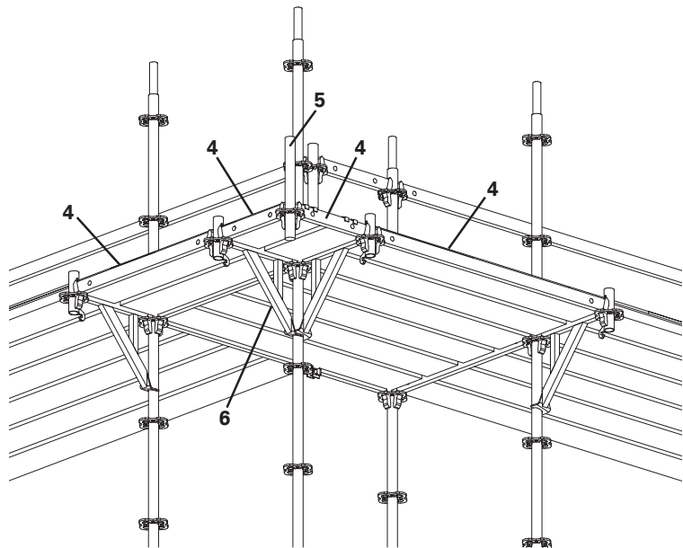
Fig.C3-3b Corner view from below
