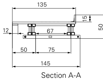
Section A-A Fig. B2.13a
