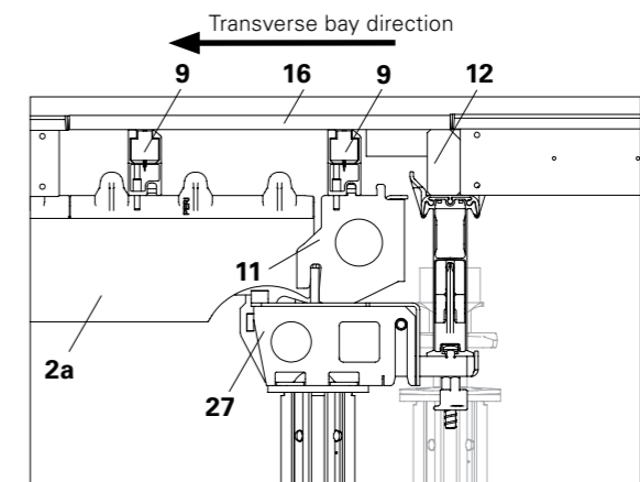
Section B-B with filler timber
