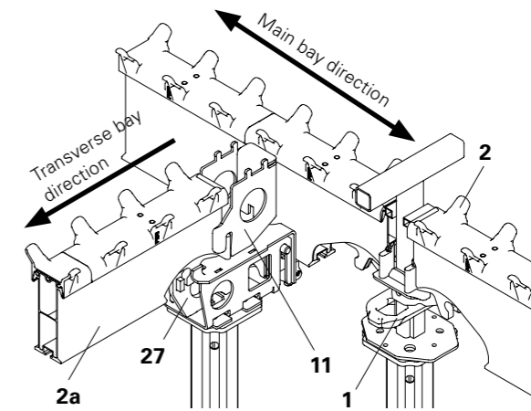
Detail X without filler timber
